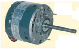
5.5" PSC 6 Pole Furnace Blower Motor (1/2 HP, 115V, 1075 RPM) MAR03587 Sale $98.09
