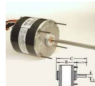
Condenser Motor 1/4HP 208/230V 1075RPM ICPF257-3728 Sale $45.71
