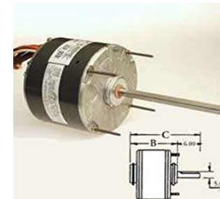
1/6HP 208/230V, 1075RPM Reverse Rotation ICPF257-3727 Sale $43.91
